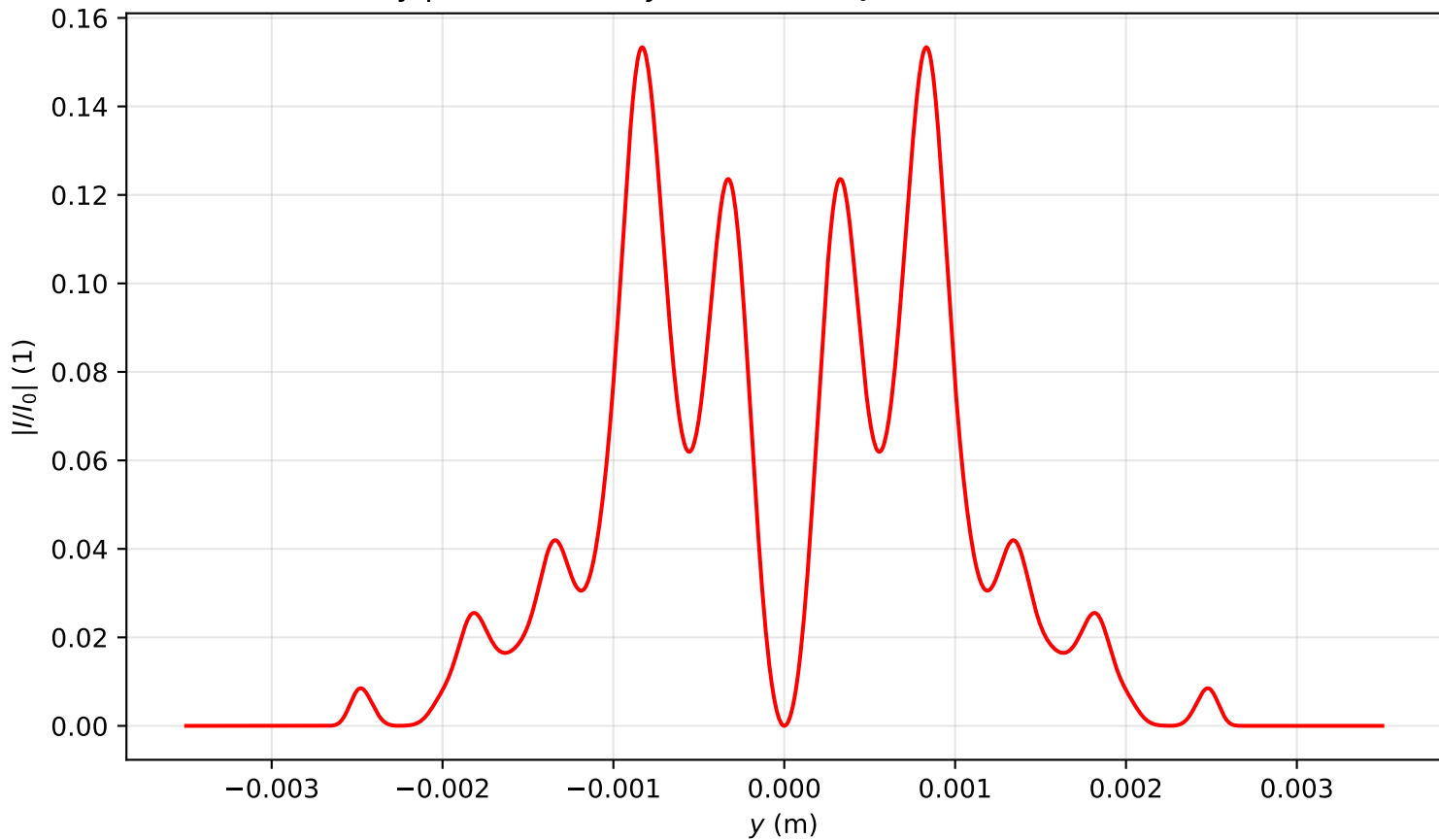
Intensity profile I(x=0, y, z=3.503)/I_0 , P_{in}=8.0P_{cr} , artificial time
